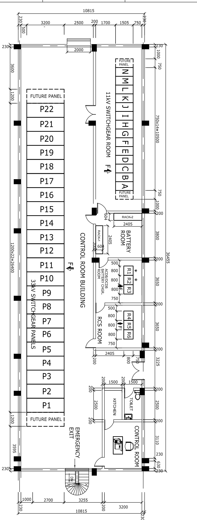
PANEL DESCRIPTION FOR 33KV SWITCHGEAR
